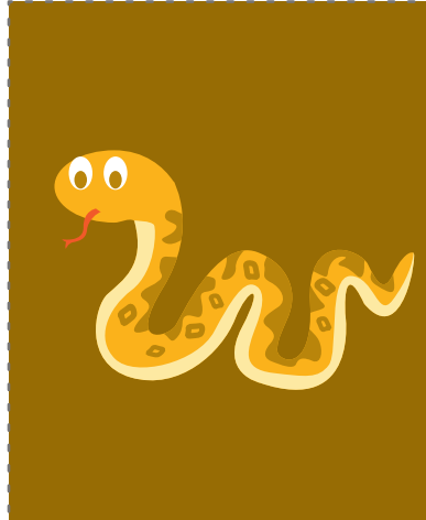
Python
